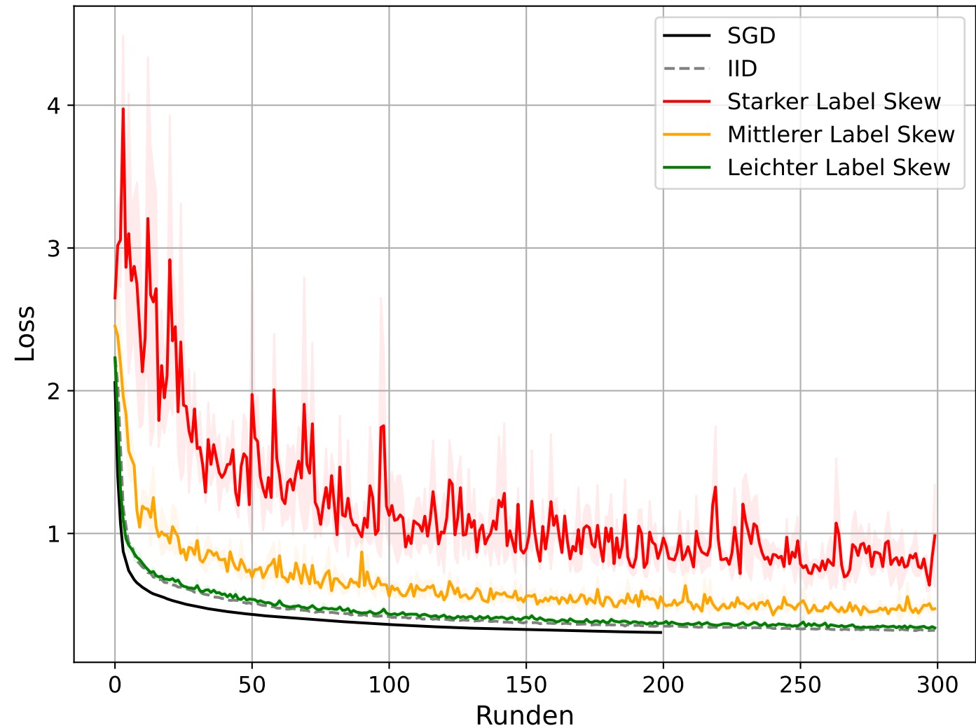
Label Skew Loss
